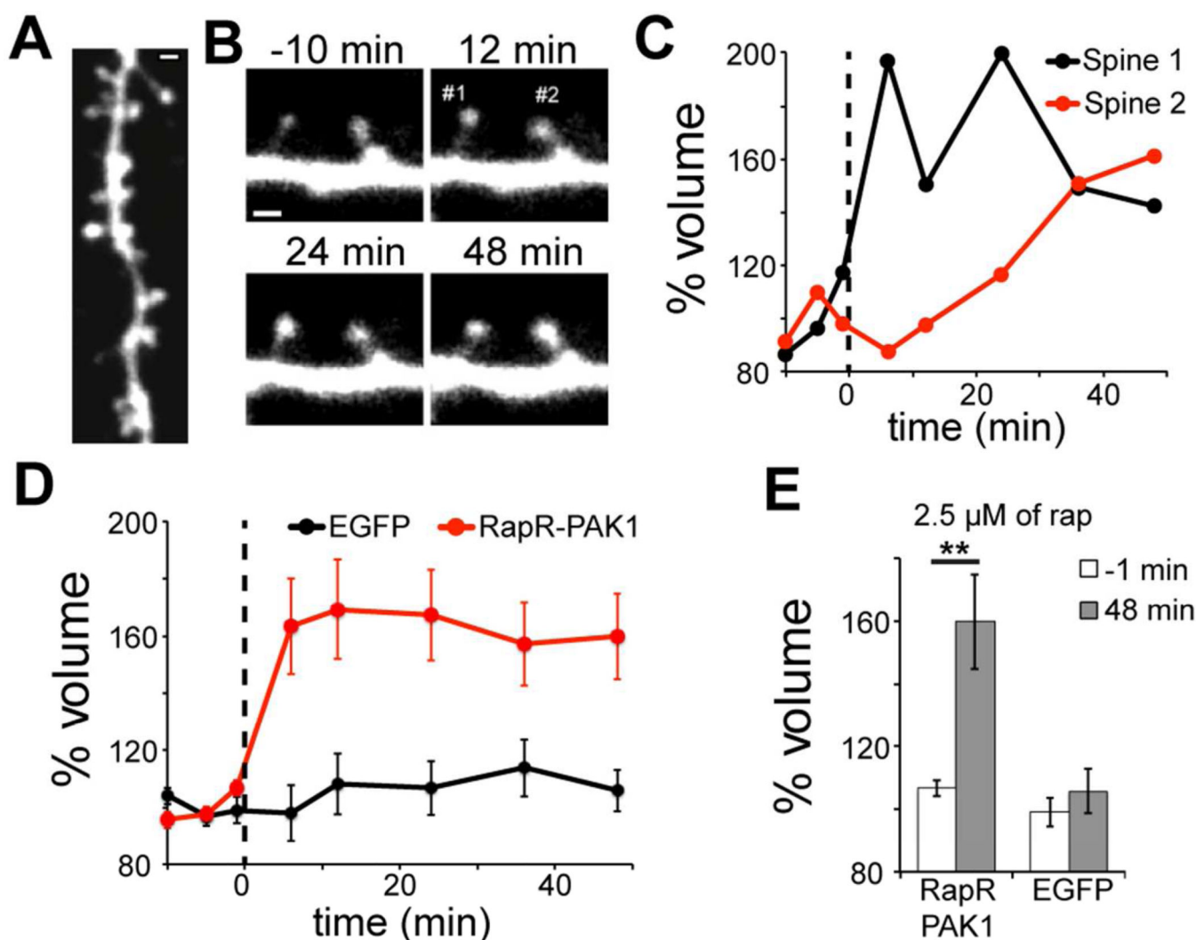
Figure 2. Enlargement of dendritic spines induced by rapamycin
