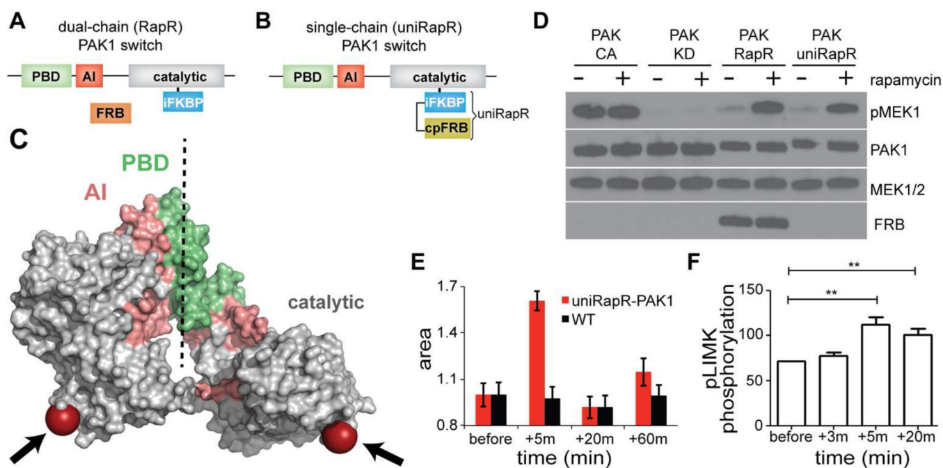
Figure 1. Engineering rapamycin-responsive PAK1 analogs
