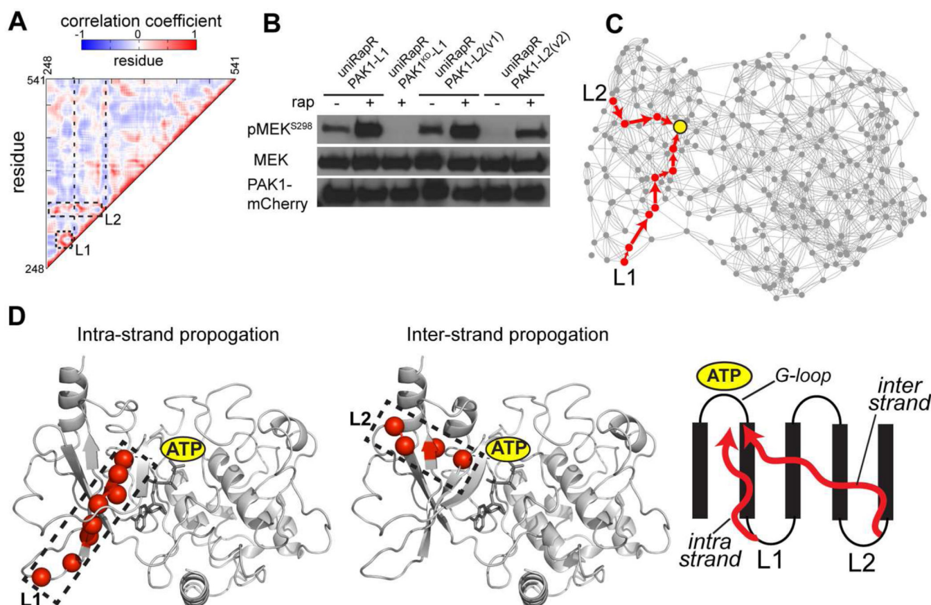
Figure 3. Understanding the mechanism of allosteric propagation to generate PAK1 analogs (A) Correlative motions of residues in the PAK1 kinase domain, computed by discrete molecular dynamics. Red and blue denote correlation and anti-correlation between two residues, respectively. (B) Insertion of uniRapR into both identified insertion sites conferred control by rapamycin. In the second version of the L2-based analog (uniRapRPAK1-L2-v2), the loop residues from PAK1 were removed, resulting in tighter control. (C) Network representation of the kinase domain based on residue-residue contacts (<5.5Å). Gray nodes represent residues; edges represent the contacts between \alpha -carbons. L1 and L2 insertion sites are shown. Red arrows represent the propagation pathways from the insertion loop to the ATP binding site (yellow node). (D) Suggested mechanism of PAK1 switching generated using L1 loop (left) and L2 loop (middle). Illustration of the mechanisms of PAK1 analogs (right). The perturbation is transmitted from L1 and L2 to the G-loop through intra- and inter-strand pathways, respectively.
